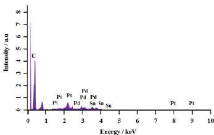
Fig .3.EDX spectra of a) Pt–Sn–Pd/MC.
