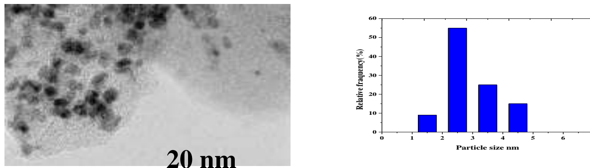
Fig. 2. Tem images for the prepared catalyst Pt–Sn–Pd/MC.
