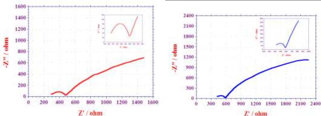
Fig 2: AC impedance spectra of carbon steel immersed in various test solutions (Nyquist plots)
